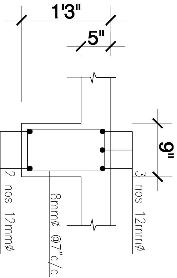
BEAM (B1)
